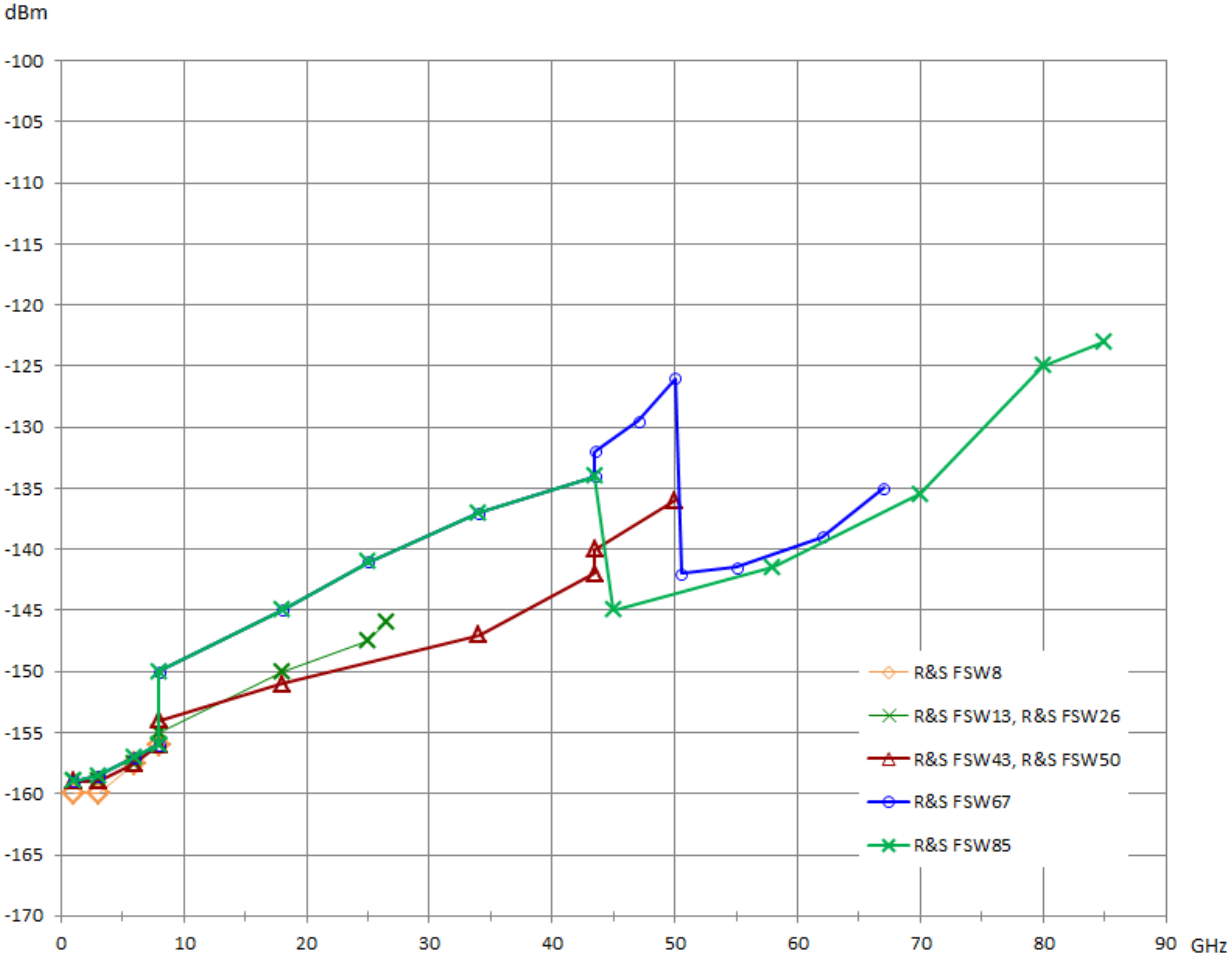
Typical displayed average noise level of the R&S®FSW models 9 for f > 1 GHz without R&S®FSW-B24 RF preamplifier option.
