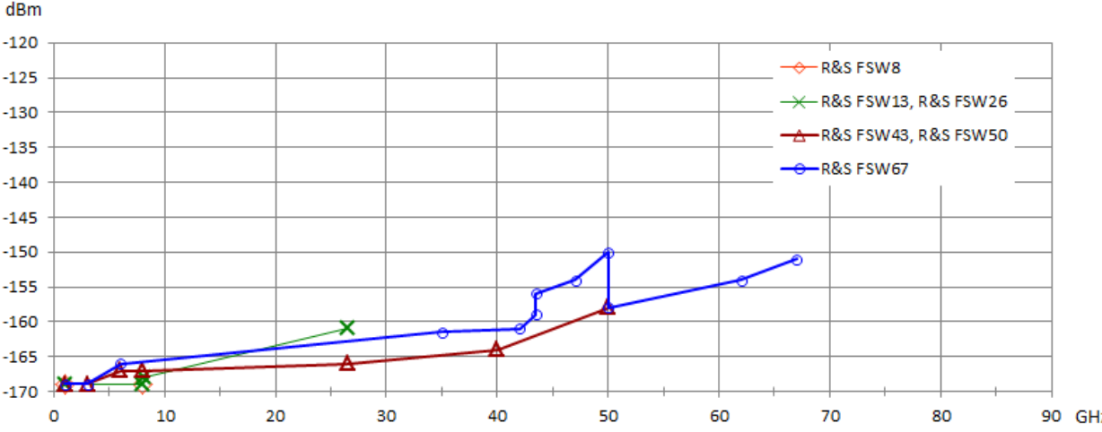
Typical displayed average noise level of the R&S®FSW models 9 for f > 1 GHz with R&S®FSW-B24 10 RF preamplifier option, preamplifier gain = 30 dB.
